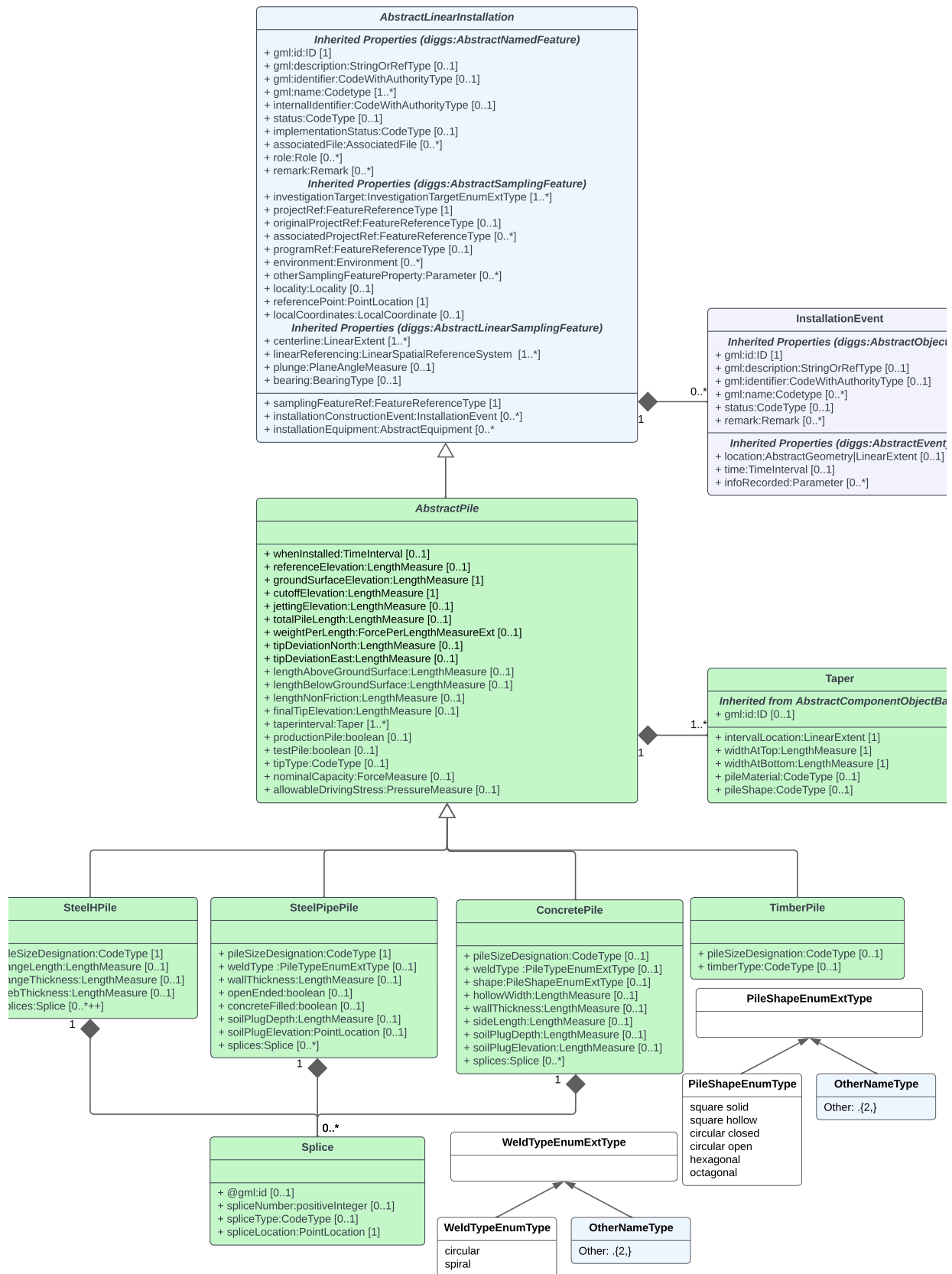
Figure 1. UML diagram illustrating the proposed objects for defining pile installation objects and their associated objects (green). :Light-blue colored objects have been previously developed. In DIGGS, piles are Installation objects that inherit properties from AbstractInstallation, which is a child of AbstractSamplingFeature, the parent object of all sampling features. See text for further discussion
